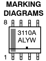
SO-8 D SUFFIX CASE 751
