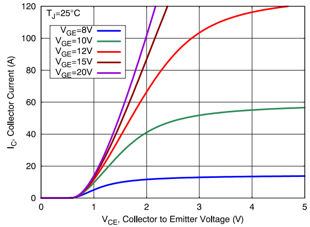
Figure 2. Output Characteristics
