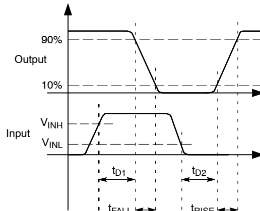
Figure 4. Inverting
