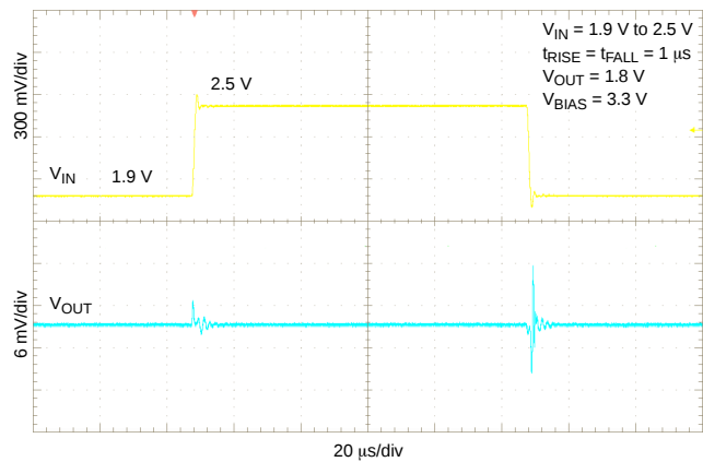
Figure 30. IN Line Transient Response – I_{OUT} = 1 \text{ A}
